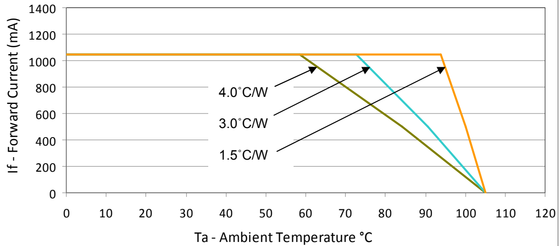
Figure 33: Derating Curve for BXRA-W0802, BXRA-N0802, 1050mA Drive Current
